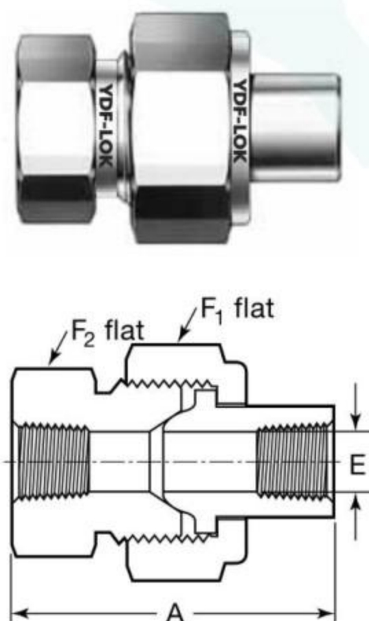
联合球形活接头 (Union Ball Joints)
