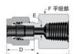
Bulkhead Female Connector 14
