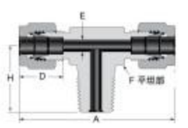
Male Run Tee 28
