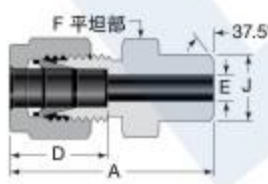
Equal Union 17
