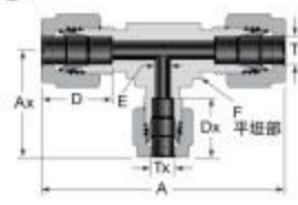
Male Branch Tee 27
