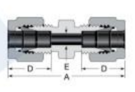
Reducing Union 18
