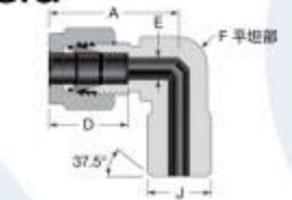
Elbow Tube Socket Weld 23
