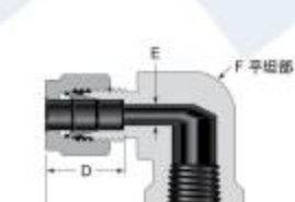
Female Elbow 24
