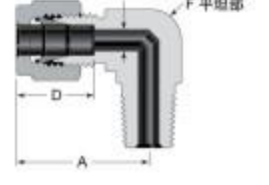
Male Elbow 23
