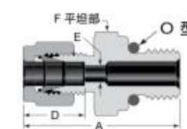
Male Connector G Thread 11
