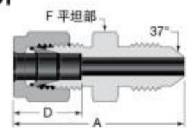
Union Elbow 20
