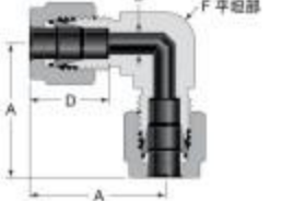
Male Elbow 21
