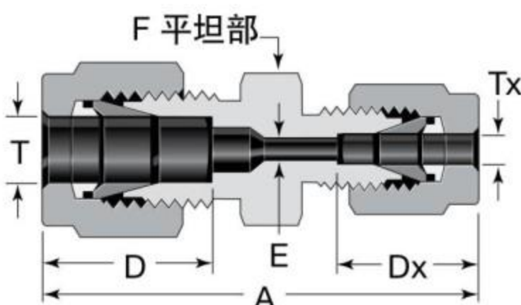
公制Tube管 metric Tube to fractional tube
