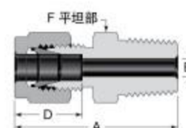
Male Connector G Thread - G Type 8
