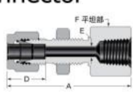
Bulkhead Male Connector 15
